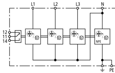
Basic circuit diagram DSH TT 255 FM
