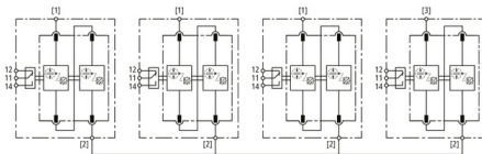
Basic circuit diagram DV M2 880 FM
