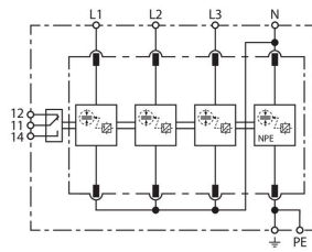
Basic circuit diagram DV M2 TT 255 FM
